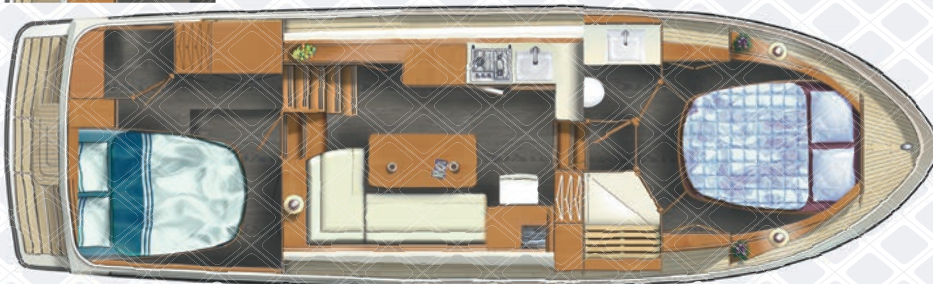
Layout Grand Sturdy 35.0 AC
