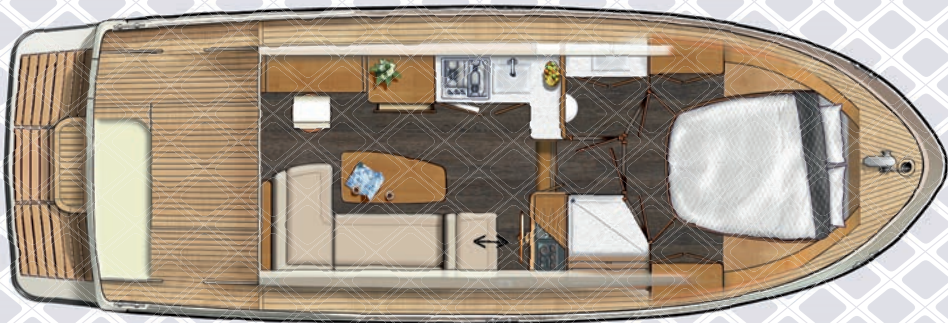
Layout Grand Sturdy 30.0 Sedan
